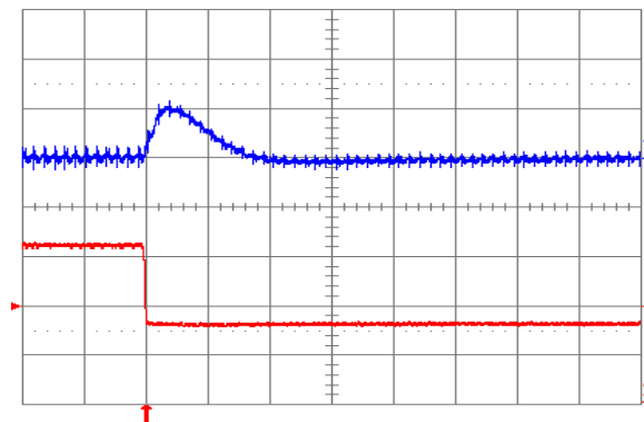
Fig. 2.0V.7: Output voltage response for V_{out} = 2.0 V to negative load current step change from 16 A to 8 A with slew rate of -5 \text{ A}/\mu\text{s} at V_{in} = 12 V. Top trace: output voltage (200 mV/div.); Bottom trace: load current (5 A/div.). C_o = 100 \mu\text{F} ceramic. Time scale: 20 \mu\text{s}/\text{div} .
