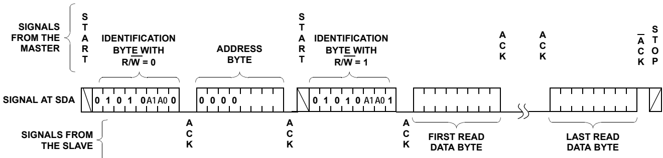
FIGURE 19. READ SEQUENCE
