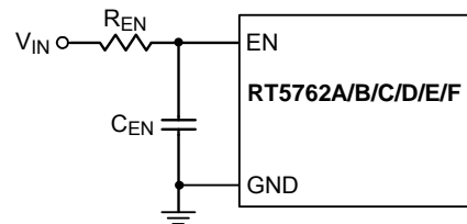
Figure 6. Enable Timing Control
