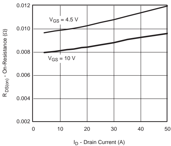
V_{GS} = 4.5\text{ V} V_{GS} = 10\text{ V} I_D - Drain Current (A)
