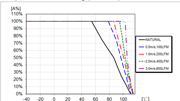
Available load current vs. ambient air temperature and airflow at V_i = 48 V. See Thermal Consideration section.
