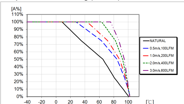
Available load current vs. ambient air temperature and airflow at V_i = 9 V. See Thermal Consideration section.
