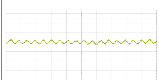
Output voltage ripple at: T_{P1} = +25^{\circ}\text{C} , V_i = 48\text{ V} , I_o = 3.33\text{ A} resistive load. Trace: output voltage (20 mV/div.). Time scale: (5 \mu\text{s} /div.).
