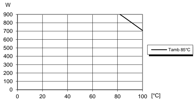
Available load current vs. base plate temperature. V_I = 54\text{ V} . See Thermal Consideration section.
