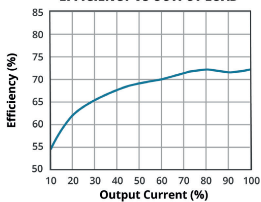
EFFICIENCY VS OUTPUT LOAD
