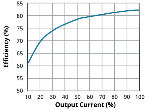
EFFICIENCY VS OUTPUT LOAD AE10-EW-S24
