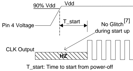
Figure 1. Startup Timing
