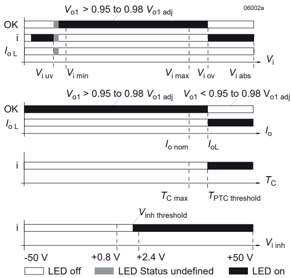
Fig.8 LED indicators
