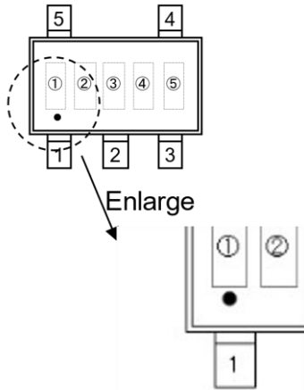
SOT-25(with Under dot mark ①)
