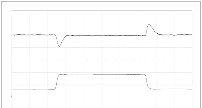
Output voltage response to load current step change (3–9–3 A) at V_i = 12\text{ V} , C_o = 3 \times 100\ \mu\text{F} + 270\ \mu\text{F}/10\text{m}\Omega . Default compensation settings. Scale: 50 mV/div, 5 A/div, 50 \mu\text{s} /div.
