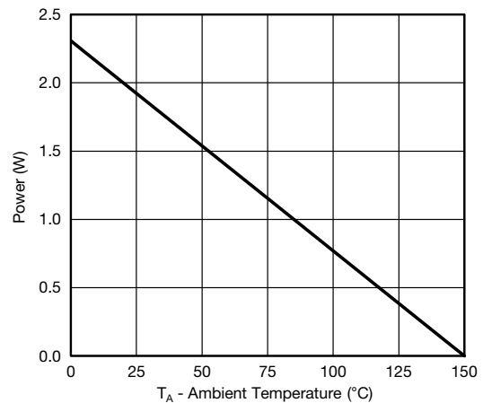
Power, Junction-to-Ambient
