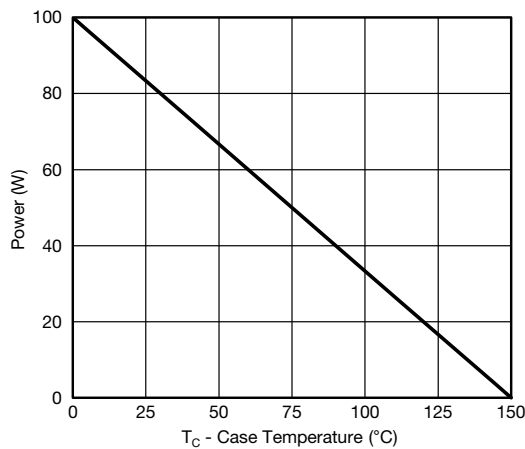
Power, Junction-to-Case
