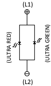
LED Schematic
