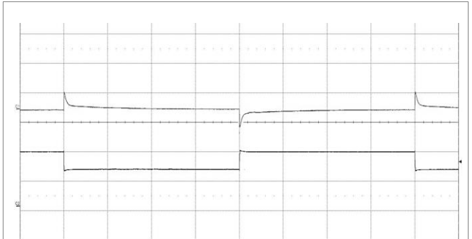
Output voltage response to load current step- change (0.625-0.937-0.625 A) at: T_{P1} = +25^\circ\text{C} , V_i = 24\text{ V} . Top trace: output voltage (500 mV/div.). Bottom trace: load current (500 mA/div.). Time scale: (2 ms/div.).
