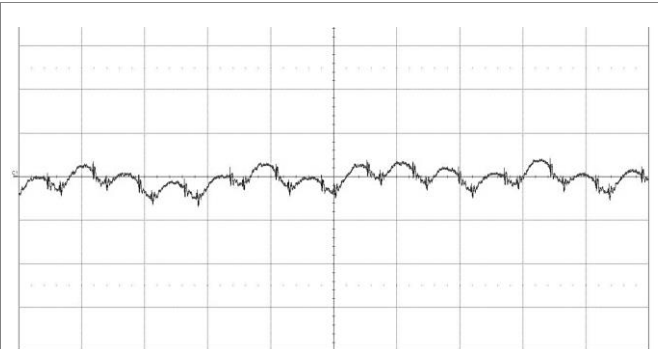
Output voltage ripple at: T_{P1} = +25^{\circ}\text{C} , V_I = 48\text{ V} , I_O = 2.5\text{ A} resistive load. Trace: output voltage (20 mV/div.). Time scale: (5 \mu\text{s} /div.). 20MHz bandwidth
