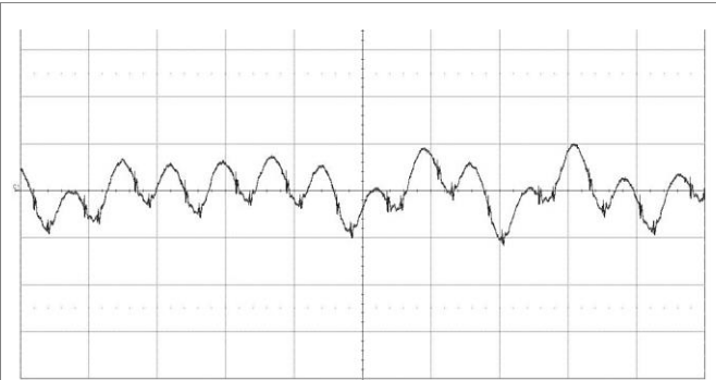
Output voltage ripple at: T_{P1} = +25^\circ\text{C} , V_I = 48\text{ V} , I_O = 2\text{ A} resistive load. Trace: output voltage (20 mV/div.). Time scale: (5 μs/div.). 20MHz bandwidth
