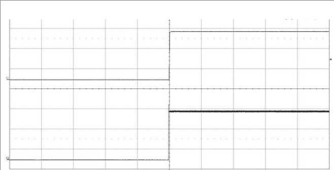
Start-up enabled by connecting V_i at: T_{P1} = +25^\circ\text{C} , V_i = 48\text{ V} , I_o = 1.25\text{ A} resistive load. Top trace: output voltage (10 V/div.). Bottom trace: input voltage (20 V/div.). Time scale: (200 ms/div.).
