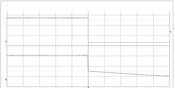
Shut-down enabled by disconnecting V_I at: T_{P1} = +25^\circ\text{C} , V_I = 48\text{ V} , I_O = 0.625\text{ A} resistive load. Top trace: output voltage (20 V/div.). Bottom trace: input voltage (20 V/div.). Time scale: (200 ms/div.).
