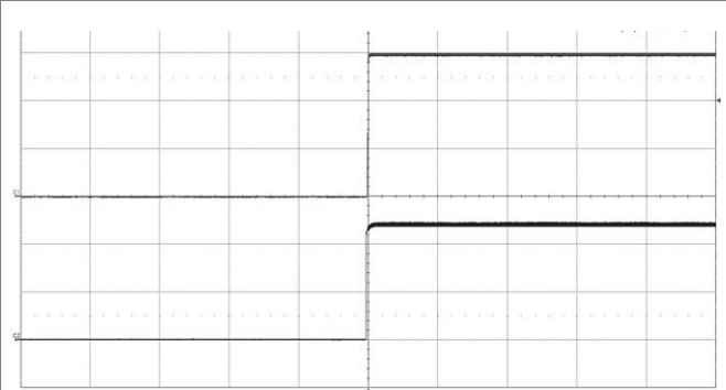
Start-up enabled by connecting V_I at: T_{P1} = +25^\circ\text{C} , V_I = 48\text{ V} , I_O = 2\text{ A} resistive load. Top trace: output voltage (5 V/div.). Bottom trace: input voltage (20 V/div). Time scale: (200 ms/div.).
