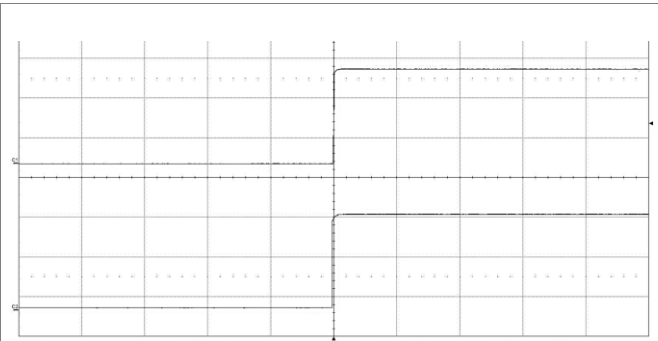
Start-up enabled by connecting V_I at: T_{P1} = +25^\circ\text{C} , V_I = 48\text{ V} , I_O = 0.625\text{ A} resistive load. Top trace: output voltage (20 V/div.). Bottom trace: input voltage (20 V/div.). Time scale: (200 ms/div.).
