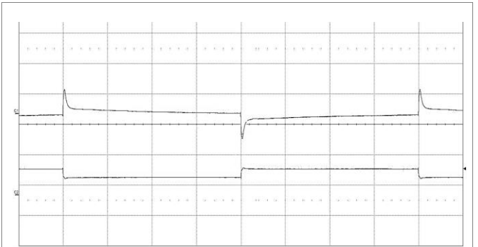
Output voltage response to load current step-change (0.312-0.468-0.312 A) at: T_{P1} = +25^\circ\text{C} , V_I = 48\text{ V} . Top trace: output voltage (500 mV/div.). Bottom trace: load current (500 mA/div.). Time scale: (2 ms/div.).
