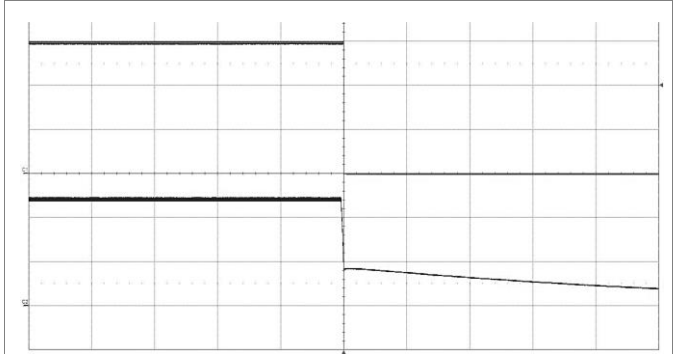
Shut-down enabled by disconnecting V_I at: T_{P1} = +25^\circ\text{C} , V_I = 48\text{ V} , I_O = 2\text{ A} resistive load. Top trace: output voltage (5 V/div.). Bottom trace: input voltage (20 V/div.). Time scale: (200 ms/div.).
