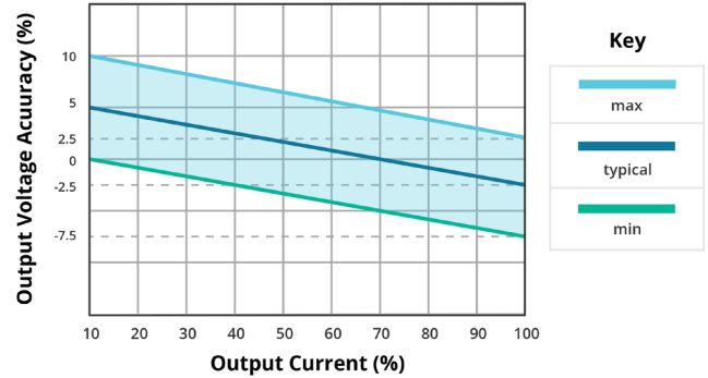
OUTPUT REGULATION CURVE 5 Vdc input / all other output models (nominal input)
