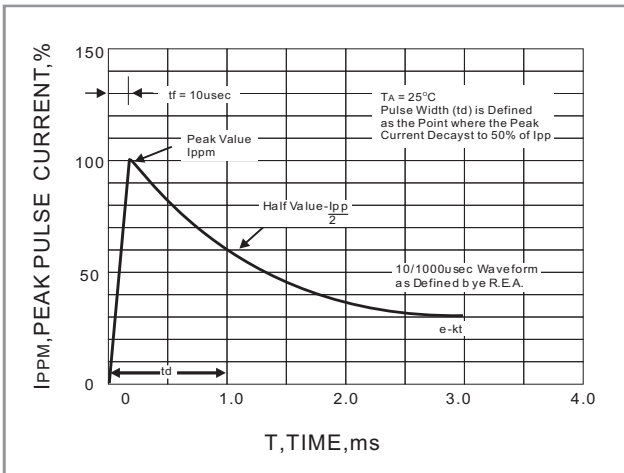
Fig.3 PULSE WAVEFORM
