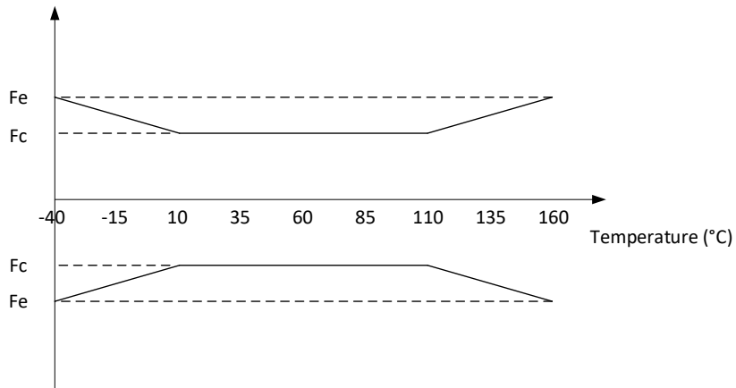
Figure 8: Pressure accuracy temperature factor
