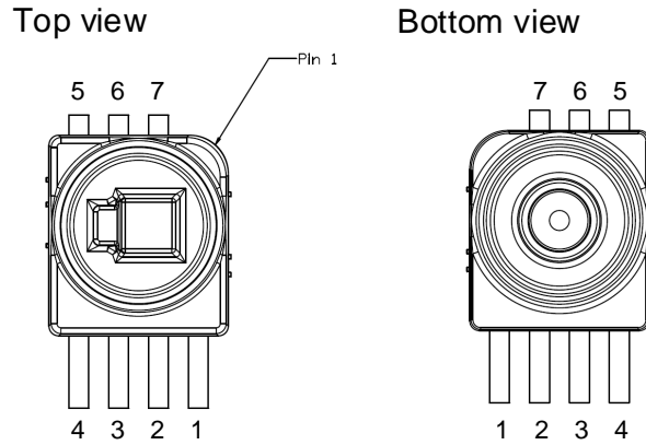
Figure 3: Package pinout
