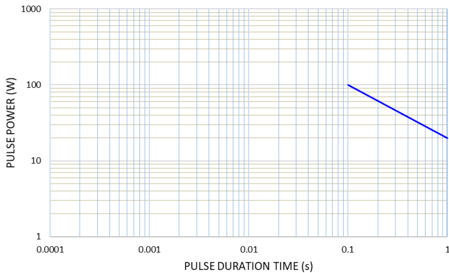
MLFM1 SINGLE PULSE (1Kohms)
