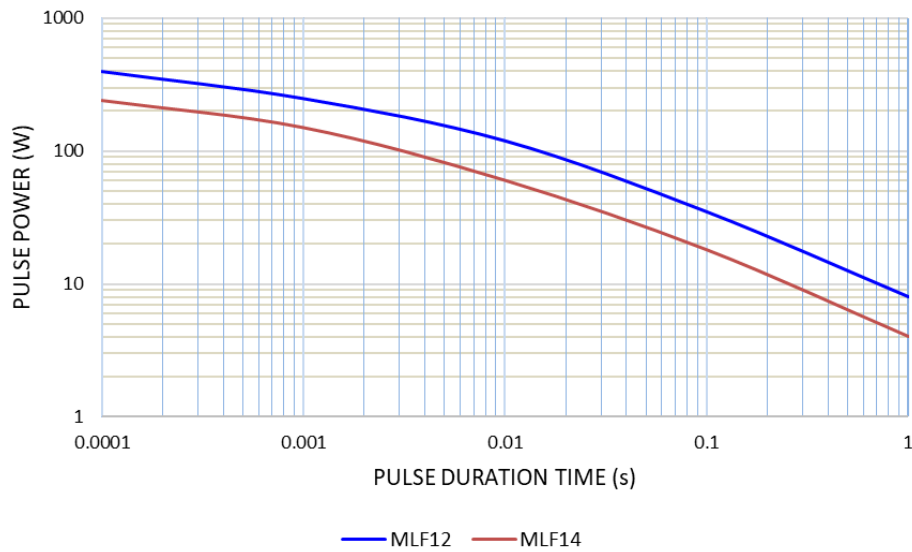
SINGLE PULSE ( R \geq 10 \text{ OHM} )
