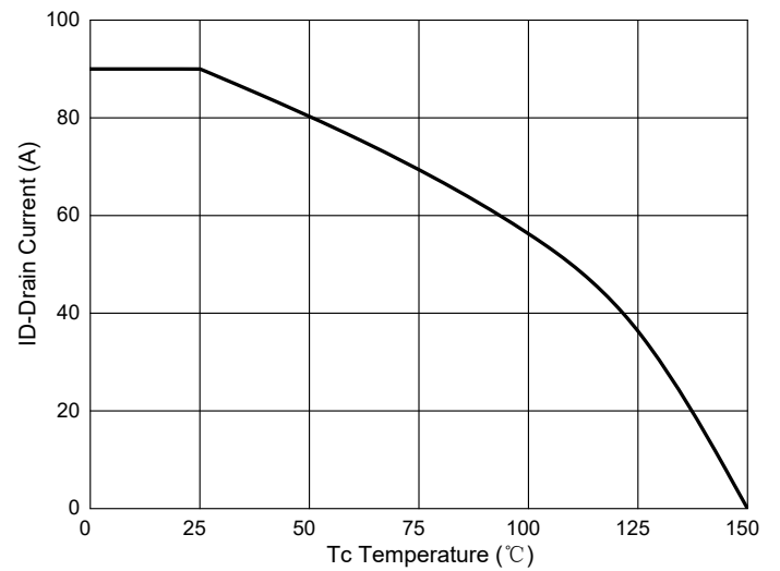
Fig. 10 - Drain Current
