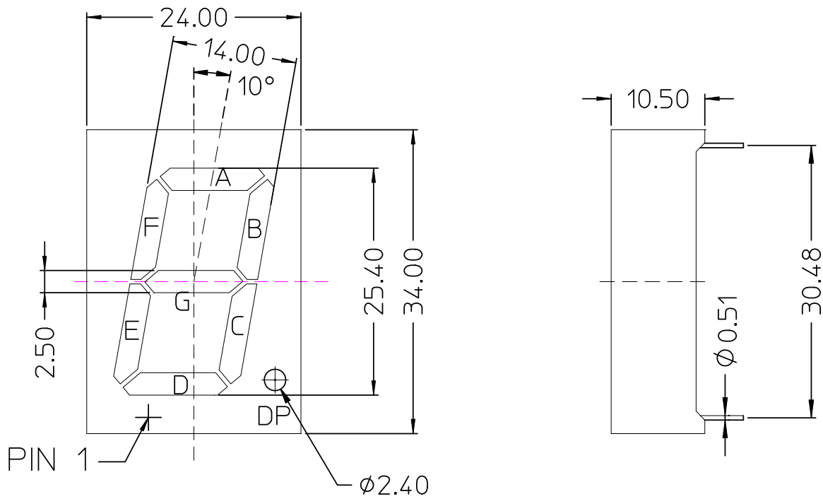
Figure 1: Package Dimension
