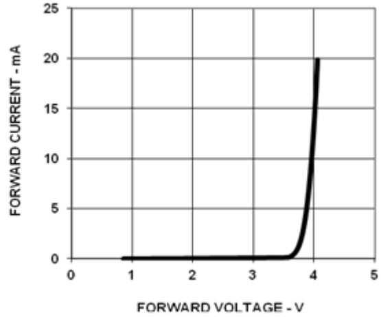
Figure 4: Forward Voltage vs. Current (Segment)
