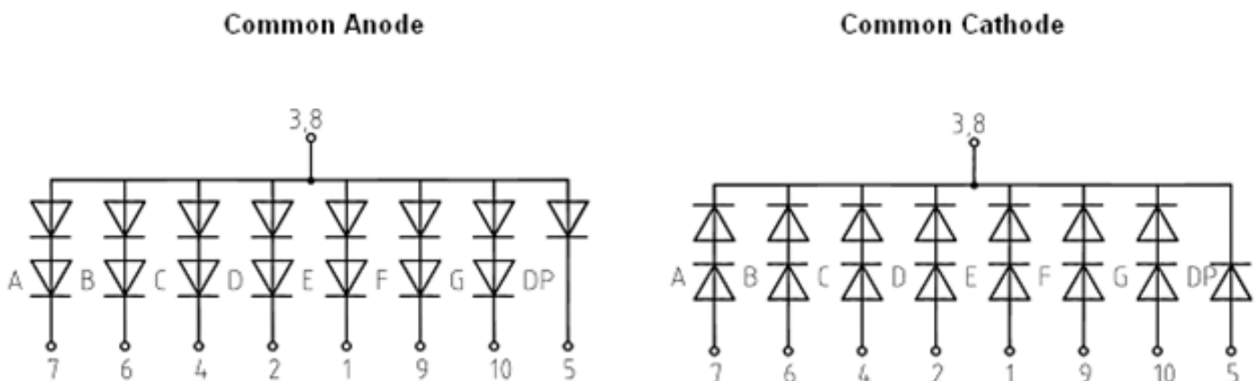
Figure 2: Circuit Diagram
