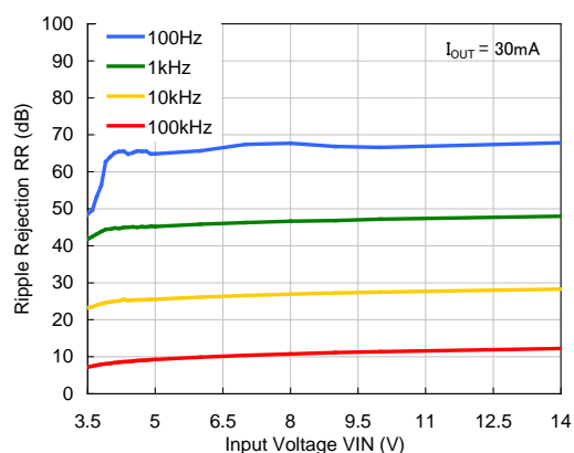
VR=3.3V, I_{OUT}=30\text{mA}
