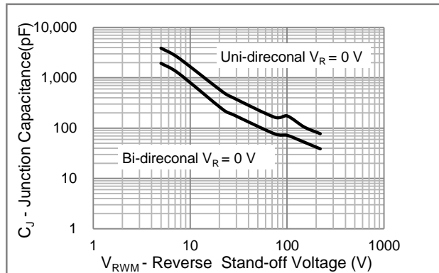
Fig.4 Typical Capacitance
