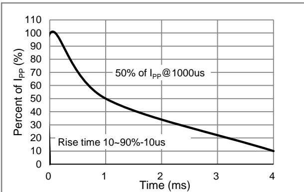
Fig.3 10/1000us Pulse Waveform
