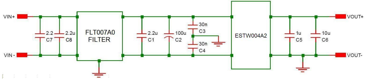
Figure 23. EMC Considerations
