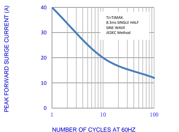
Fig.5-MAX. NON-REPETITIVE SURGE CURRENT
