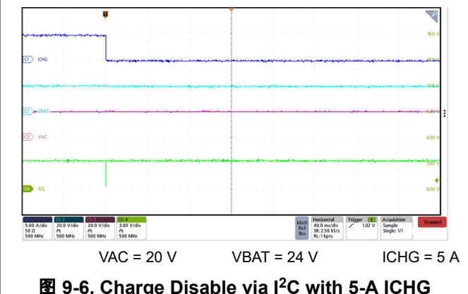
图 9-6. Charge Disable via I²C with 5-A ICHG
