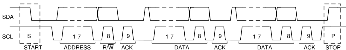
图 8-11. Complete Data Transfer on the I 2 C Bus
