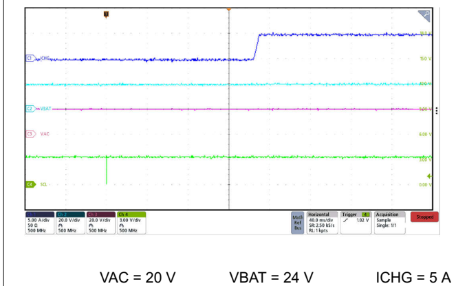
图 9-5. Charge Enable via I²C with 5-A ICHG
