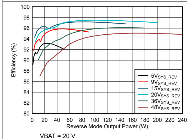
Figure 7-9. Reverse Mode Efficiency (5s battery configuration)
