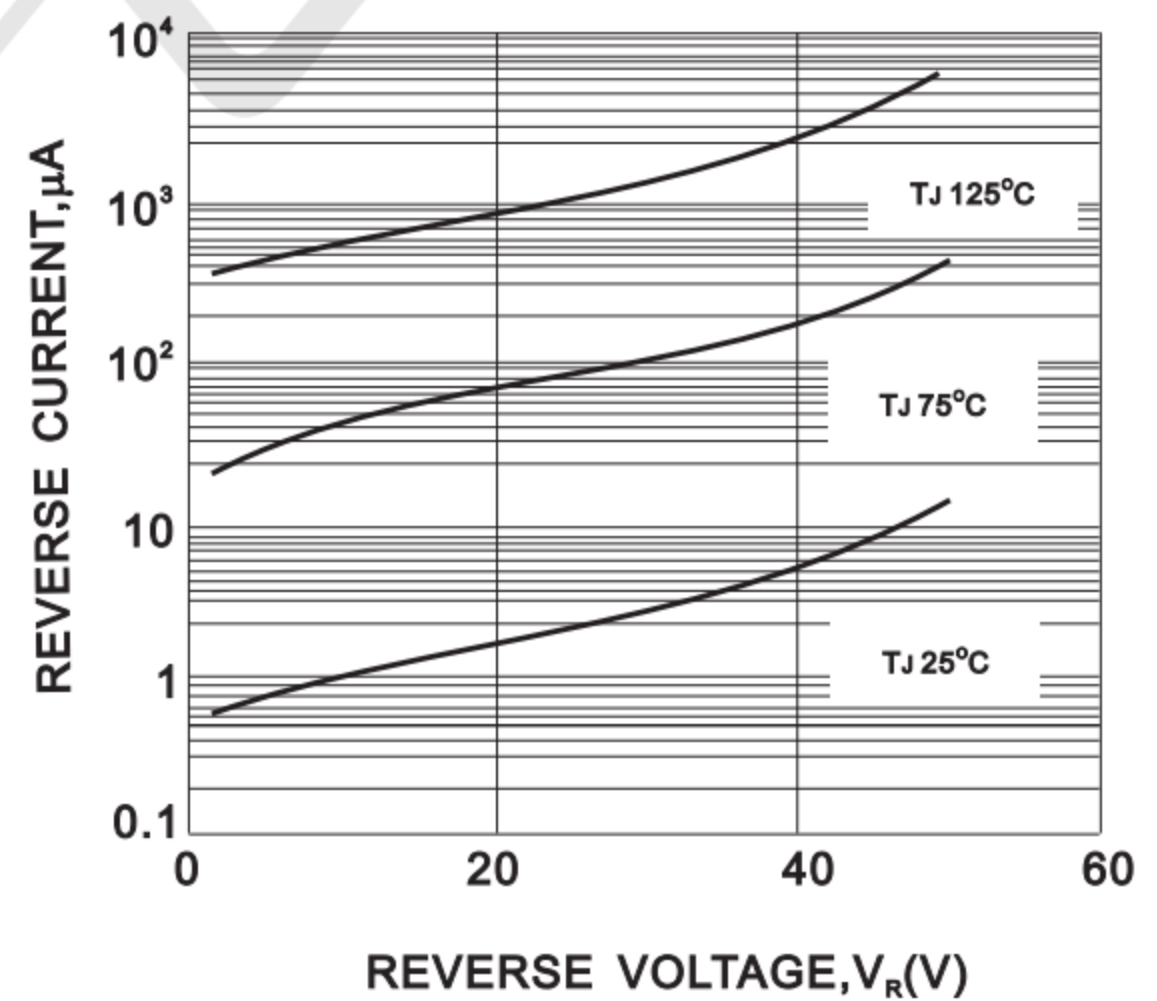
FIG. 2-TYPICAL REVERSE CHARACTERISTIC
