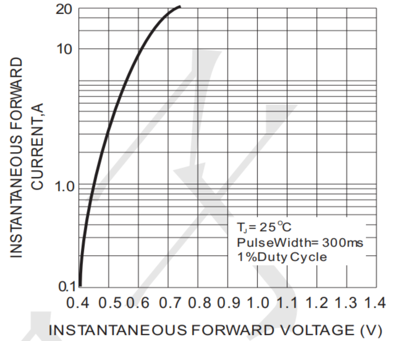
FIG. 4-TYPICAL INSTANTANEOUS FORWARD CHARACTERISTICS
