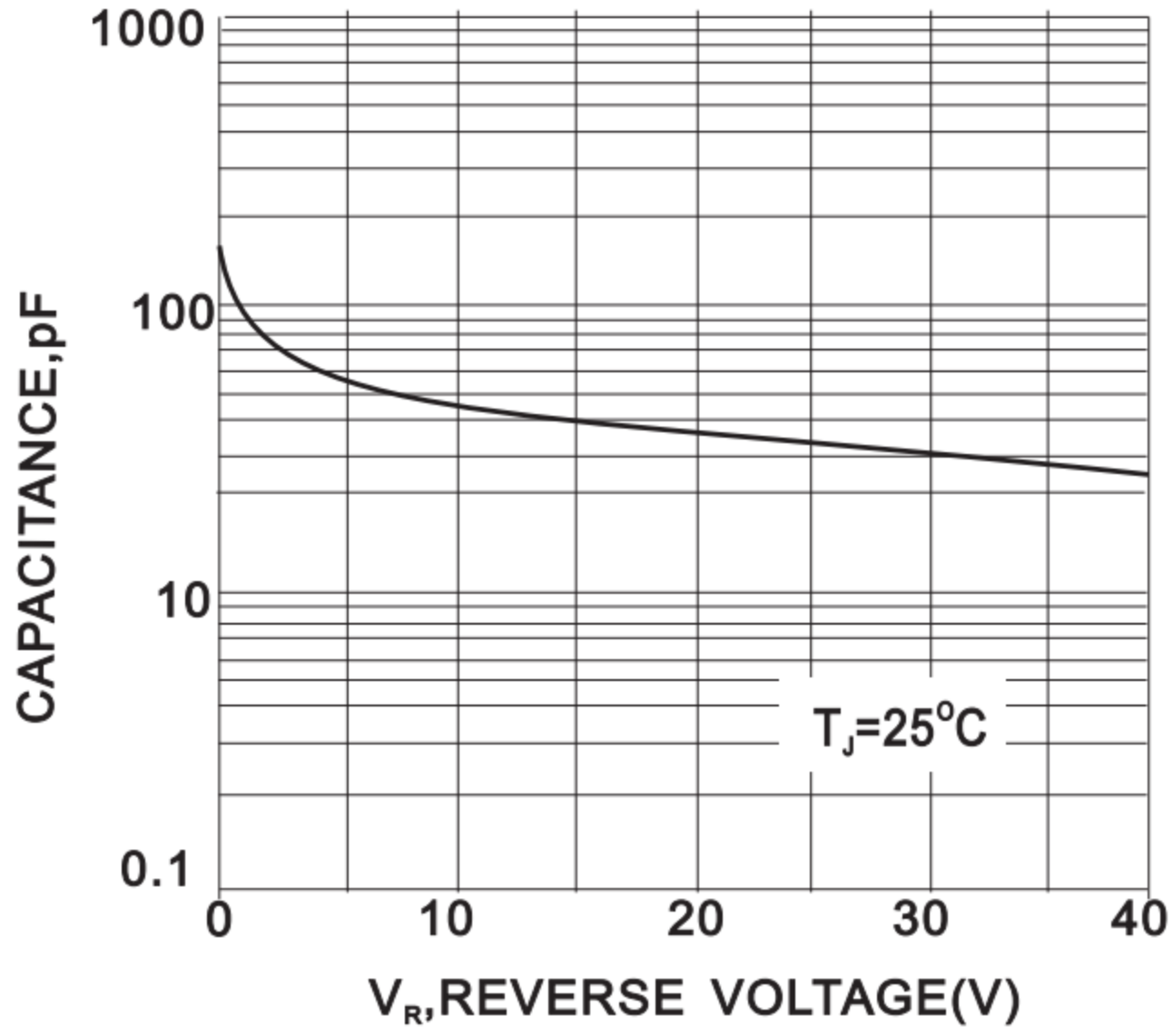
FIG. 3-TYPICAL JUNCTION CHARACTERISTIC
