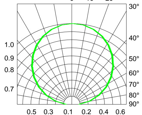
Fig.6-Radiation Diagram Ta=25°C
