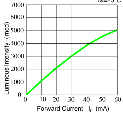
Fig.2- Luminous Intensity vs. Forward Current Ts=25°C
