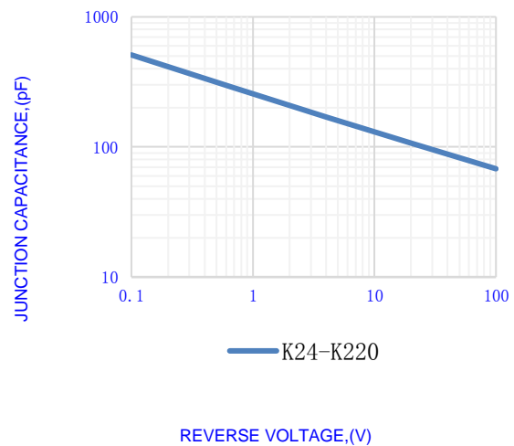
Fig.4-TYPICAL JUNCTION CAPACITANCE
