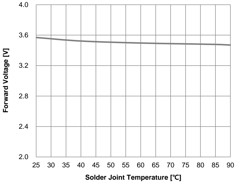
Fig 7. Solder Joint Temperature vs. Forward Voltage, I_F=180\text{mA}
