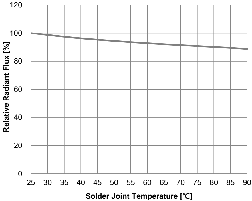
Fig 5. Solder Joint Temperature vs. Relative Radiant Flux, I_F=180\text{mA}
