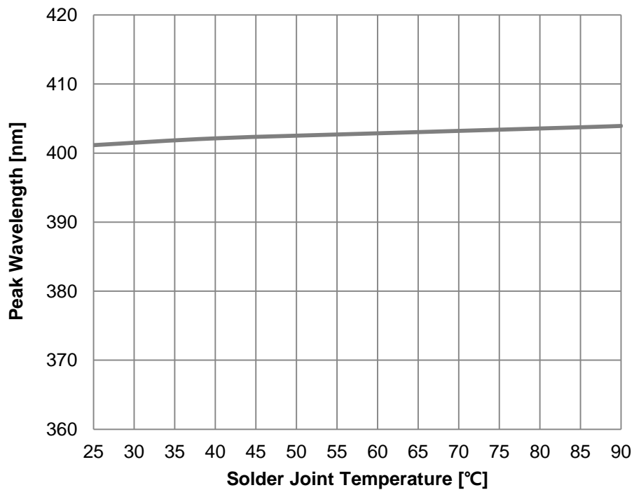
Fig 6. Solder Joint Temperature vs. Peak Wavelength, I_F=180\text{mA}
