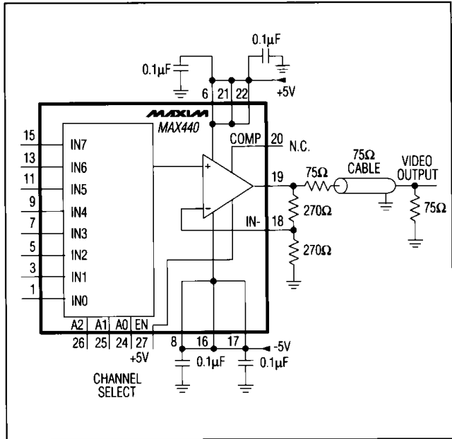
Figure 3. Coaxial-Cable Driver
