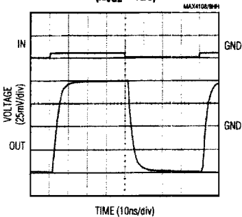
MAX4309 SMALL-SIGNAL PULSE RESPONSE ( A_{vCL} = +20 )
