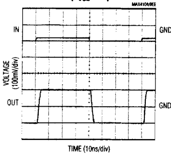
MAX4308 SMALL-SIGNAL PULSE RESPONSE ( A_{vCL} = +5 )
