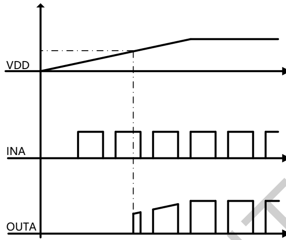
Figure 8. GBI7254 Output Vs VDD
