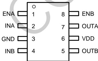
Top View (SOIC-8)
