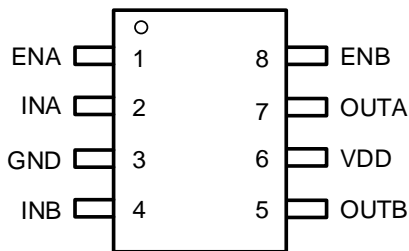
Top View (EMSOP-8)
