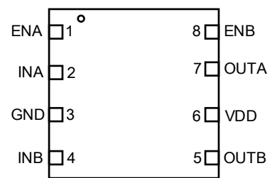
Top View (DFN3*3-8)
