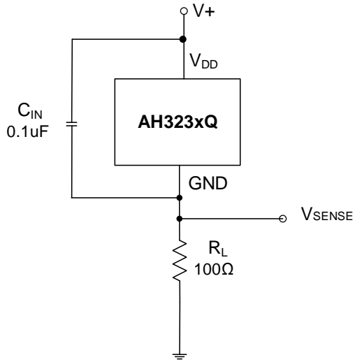
Low-side sensing
