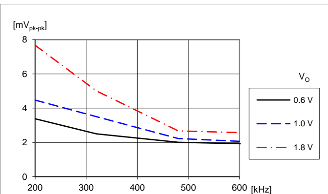
Output voltage ripple V_{pk-pk} vs. switching frequency at V_i = 12\text{ V} , I_o = \text{max } I_o , C_o = 10 \times 470\text{ }\mu\text{F}/5\text{ m}\Omega + 10 \times 100\text{ }\mu\text{F} . Frequency changed by PMBus command FREQUENCY_SWITCH.
