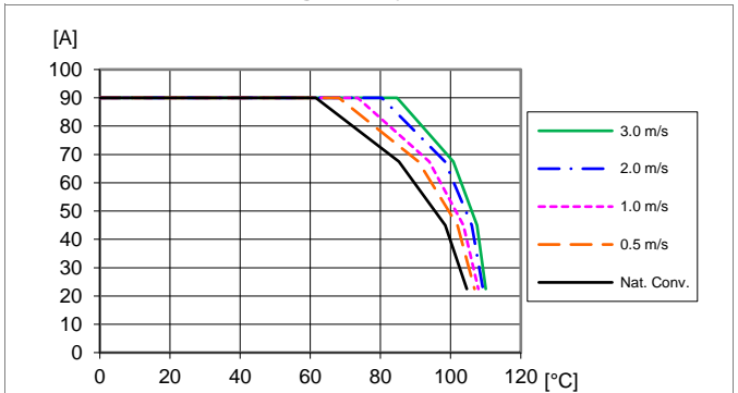
Available load current vs. ambient air temperature and airflow at V_i = 12\text{ V} . See section Thermal Consideration.
