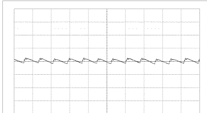
Fundamental output voltage ripple at V_i = 12\text{ V} , I_o = \text{max } I_o , C_{OUT} = 10 \times 470\ \mu\text{F}/5\ \text{m}\Omega + 10 \times 100\ \mu\text{F} . Scale: 5 mV/div, 2 \mu\text{s} /div, 20 MHz bandwidth. See section Output Ripple and Noise.
