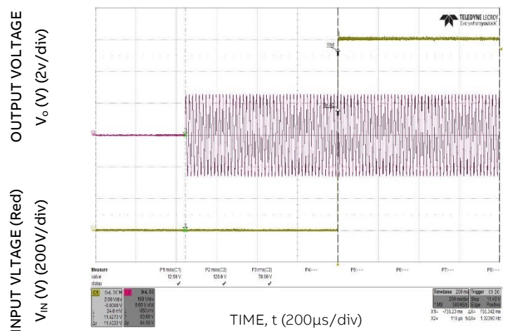
Figure 6. Typical Start-up ( V_{IN} = 230\text{Vac} , Full Load)
