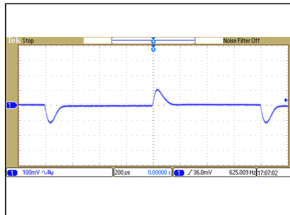
Figure 64: ATA02C36-L Transient Response Vin = 48Vdc Load: Io = 100% to 75% load change Ch 1: Vo
