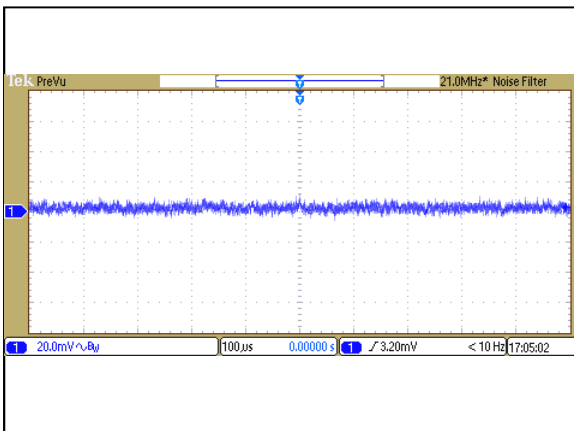
Figure 63: ATA02C36-L Ripple and Noise Measurement Vin = 48Vdc Load: Io = 0.535A Ch 1: Vo
