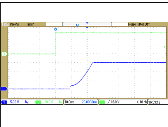
Figure 65: ATA02C36-L Output Voltage Startup Characteristic by Vin Vin = 48Vdc Load: Io = 0.535A Ch1: Vo Ch3: Vin
