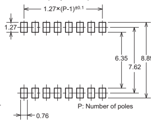
Dimensions of PCB pad (Reference) (Top View)
