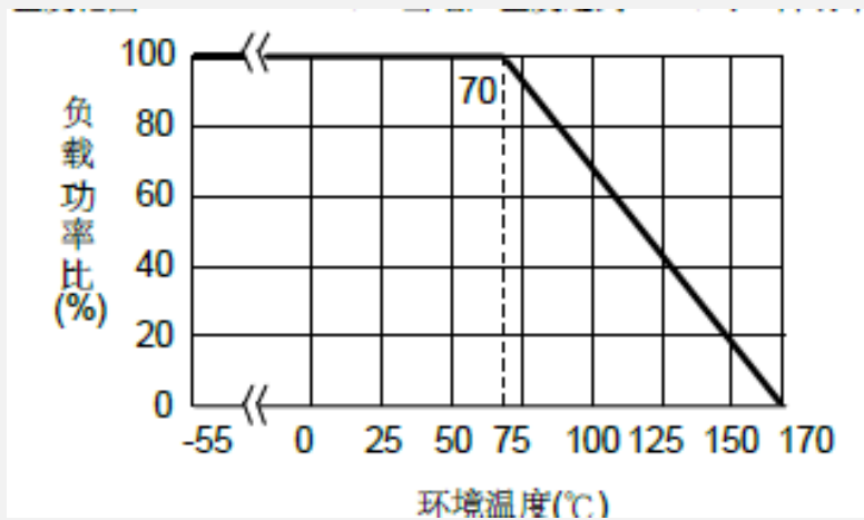
功率曲线 Power Curve
