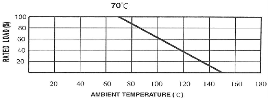
FIG.1 DERATING CURVE
