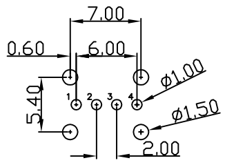
RECOMMEND PCB LAYOUT(±0.05)
