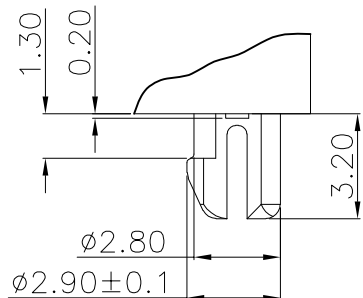
DETAIL "X" SCALE 2:1
