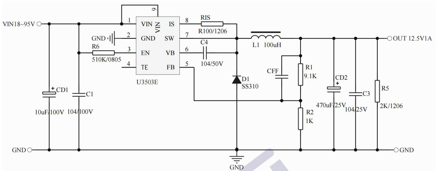
APP1: VIN = 18 ~ 95V, V OUT = 12.5V, I OUT = 1A
