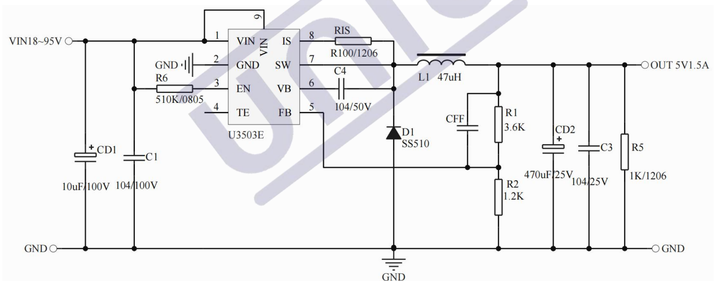
APP2: VIN = 18 ~ 95V, V OUT = 5V, I OUT = 1.5A
