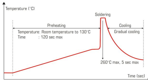
Fig.: Wave-soldering temperature-time profile to recommend
