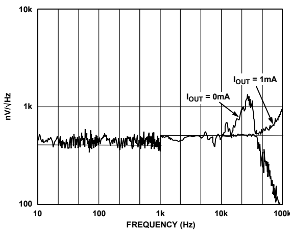
Figure 8. Noise Spectral Density
