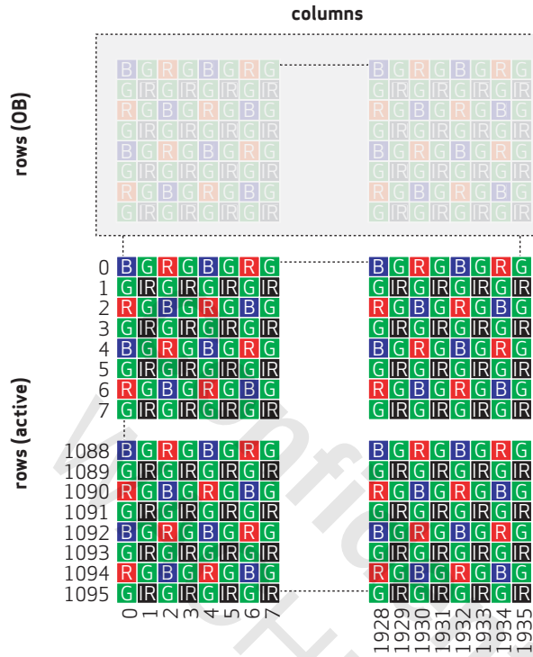
figure 3-2 pixel array region RGB-Ir filter layout
