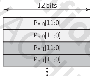
figure 5-39 2x12b DCG single HDR diagram
