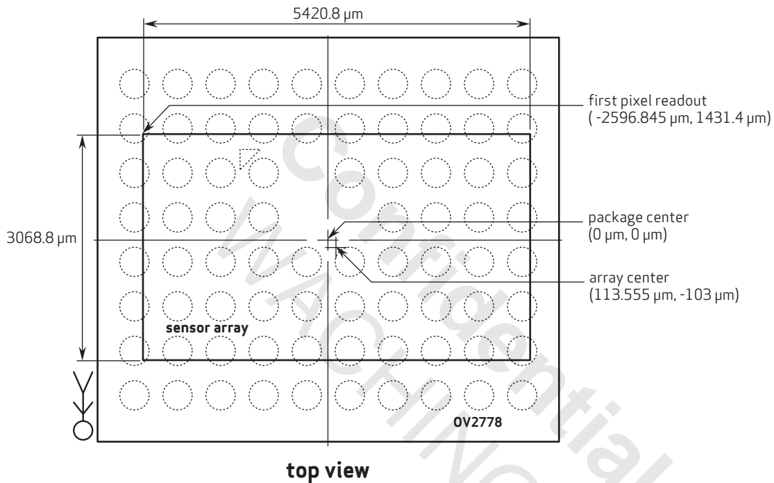
figure 10-1 sensor array center
