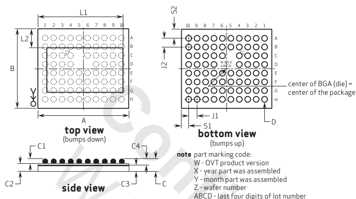
figure 9-1 package specifications
