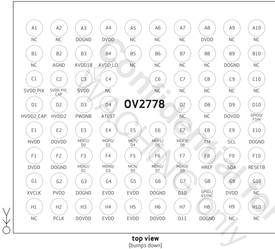
figure 1-3 pin diagram
