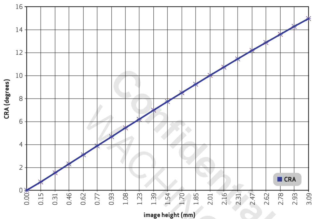
figure 10-2 chief ray angle (CRA)
