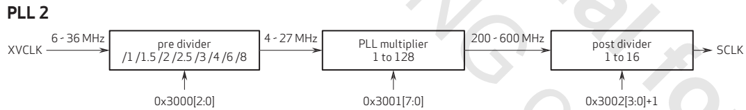
figure 3-10 PLL2 control diagram
