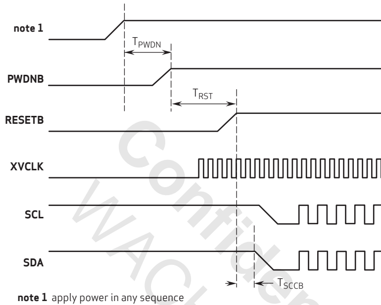
figure 1-7 power on timing diagram
