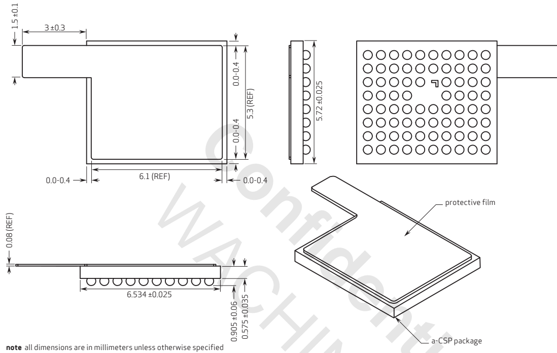
figure 9-3 protective film specifications
