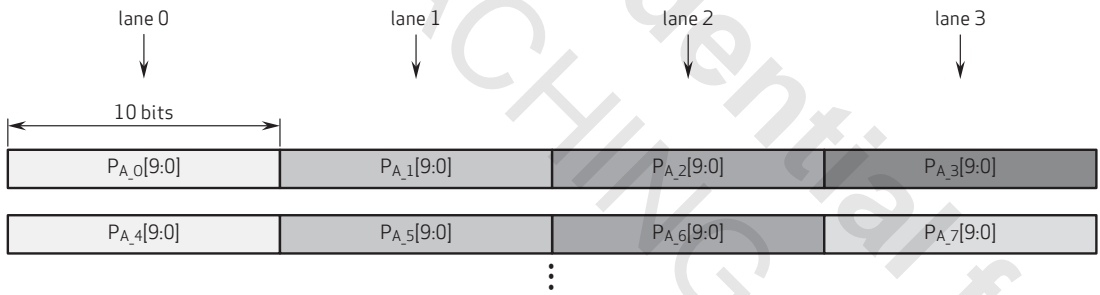
figure 5-23 10 bits linear mode diagram
