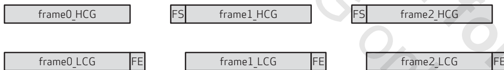
figure 5-8 non-staggered HDR without MIPI virtual channel detail diagram
