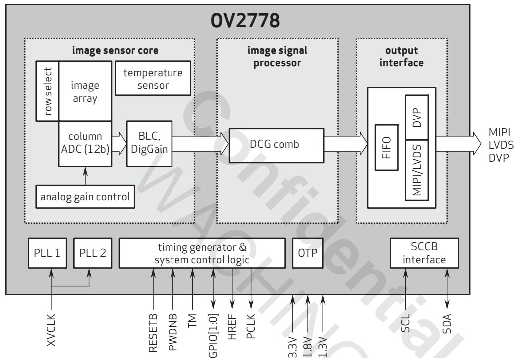
figure 2-1 OV2778 block diagram
