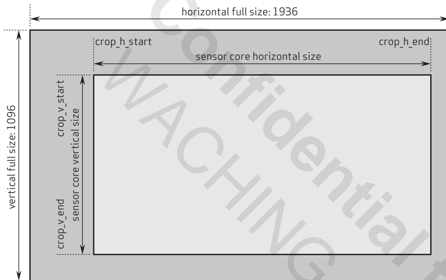
figure 3-5 pixel array access diagram
