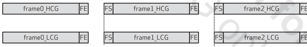
figure 5-4 non-staggered HDR with MIPI virtual channel detail diagram
