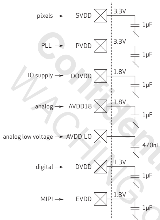
figure 1-6 OV2778 power supplies and recommended external decoupling
