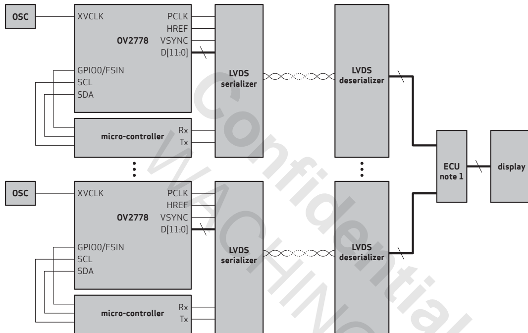
figure 1-2 multi-camera block diagram
