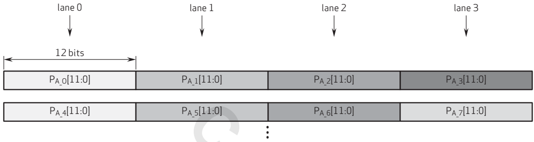
figure 5-22 12 bits linear mode diagram
