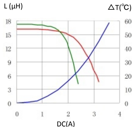
3. CD75T125NP-150KC
