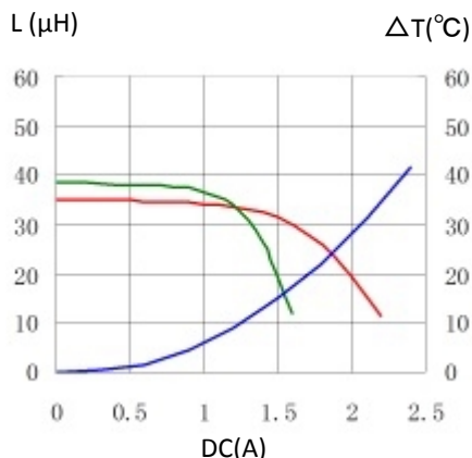
7. CD75T125NP-330KC
