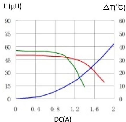
9. CD75T125NP-470KC
