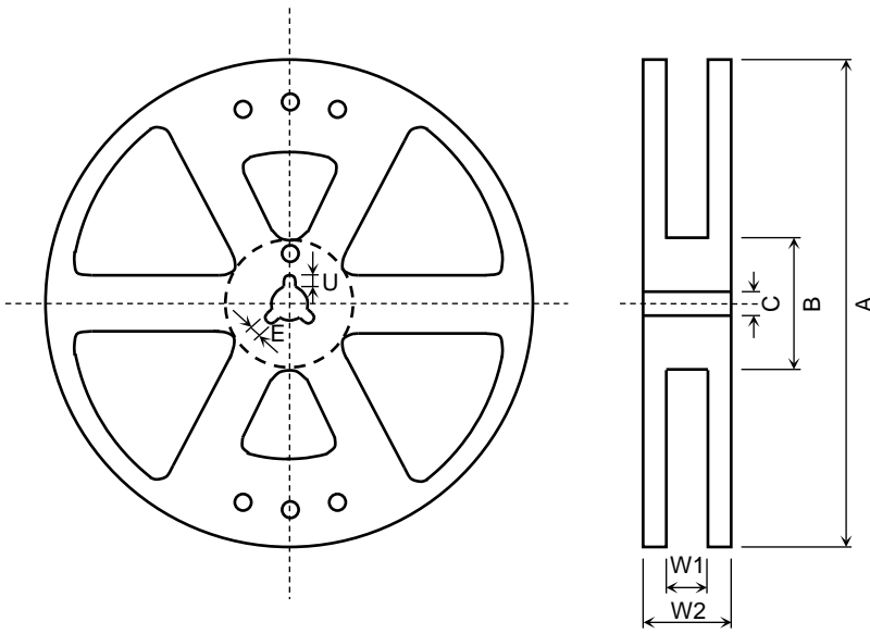
Figure 3.6.1 Reel Dimensions
