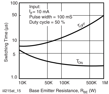
iii215at_15 Base Emitter Resistance, R_{BE} ( \Omega )
